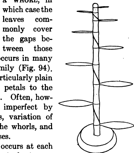
FIG. 95. — The alternate , \frac{1}{2} spiral, arrangement.
